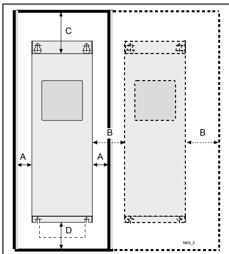
Fig. 4. NXL HVAC installation space
